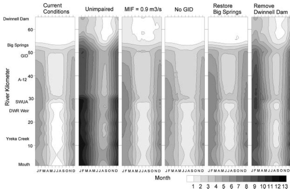
Figure 5. Simulated spatial and temporal weekly mean flow ( \text{m}^3/\text{s} )
